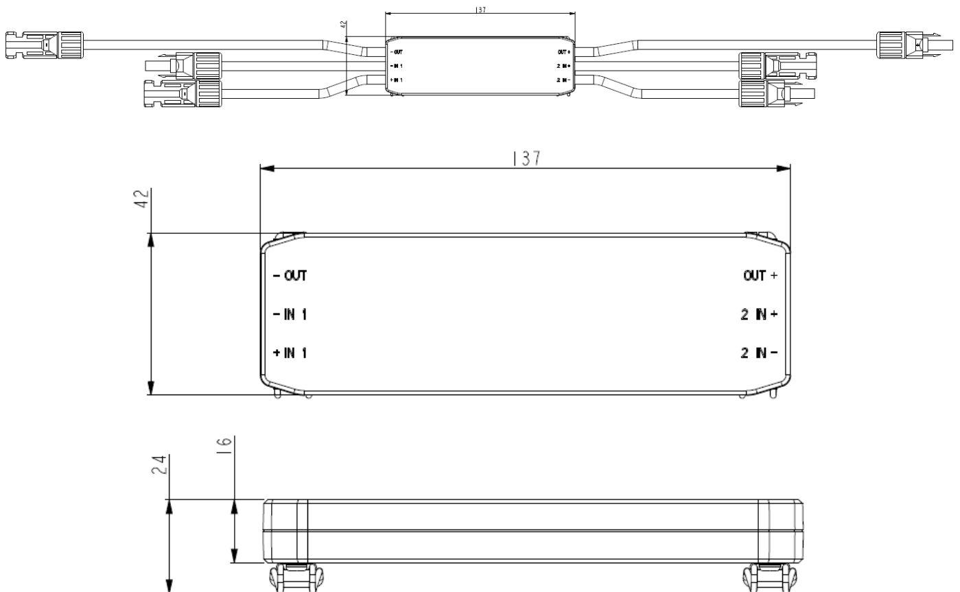
Figure 3.6&3.7&3.8 Dimensions of TSOL-RSDM-DD
