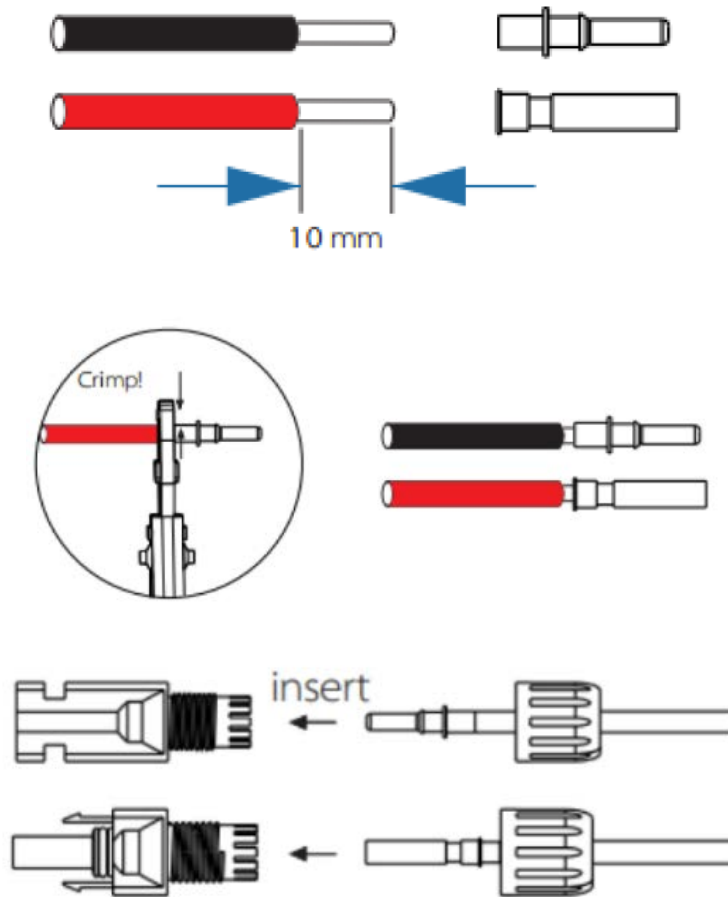
Figure 4.9&4.110&4.11&4.12 Make the DC cable
