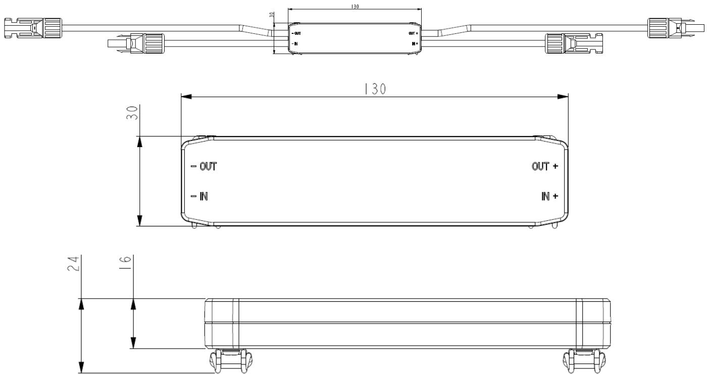
Figure 3.3&3.4&3.5 Dimensions of TSOL-RSDM-DS
