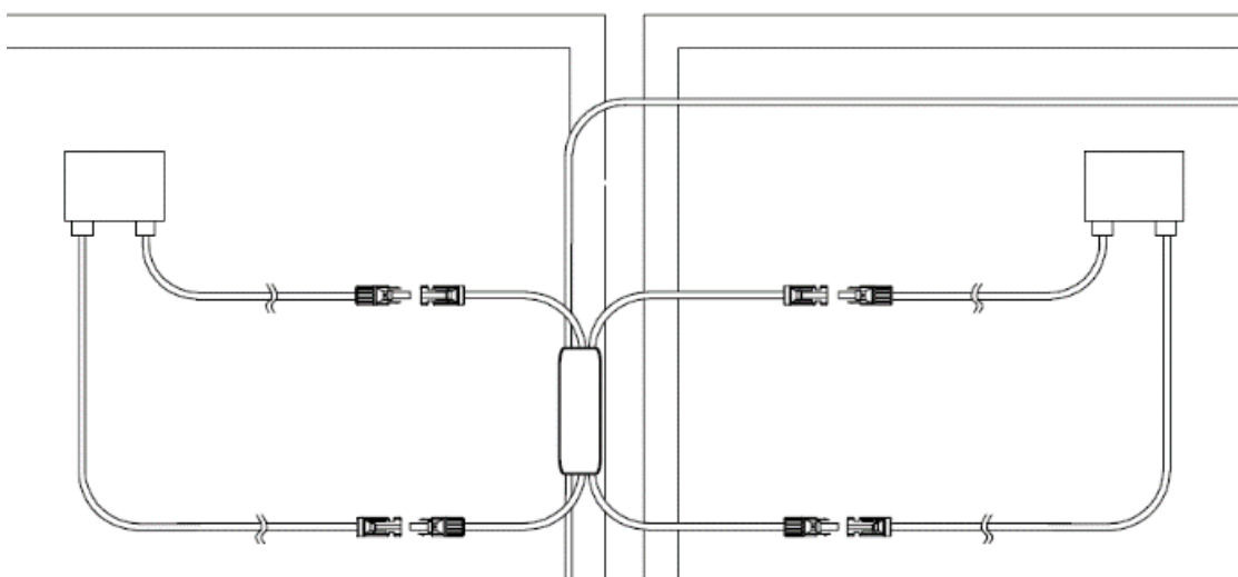
Figure 4.4 Connecting TSOL-RSDM-DD and solar modules
