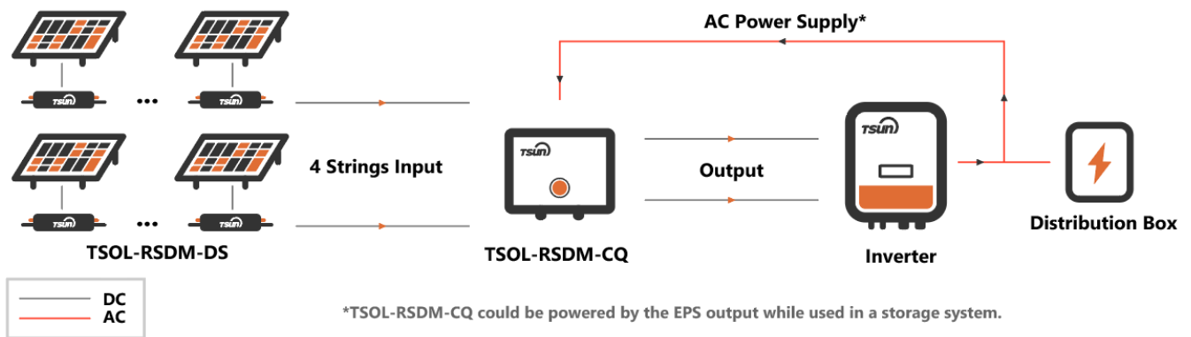
Figure 3.1 System Diagram (TSOL-RSDM-DS and TSOL-RSDM-CQ)
