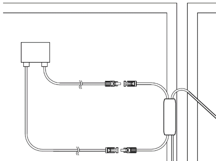
Figure 4.3 Connecting TSOL-RSDM-DS and solar module
